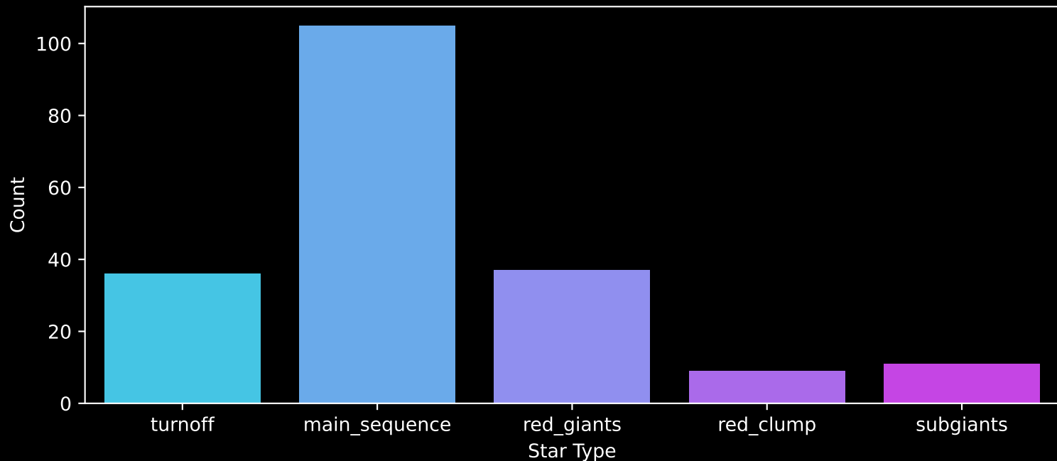
APOGEE DR17 Field: [066+47_MGA] Count plot of Star Type
