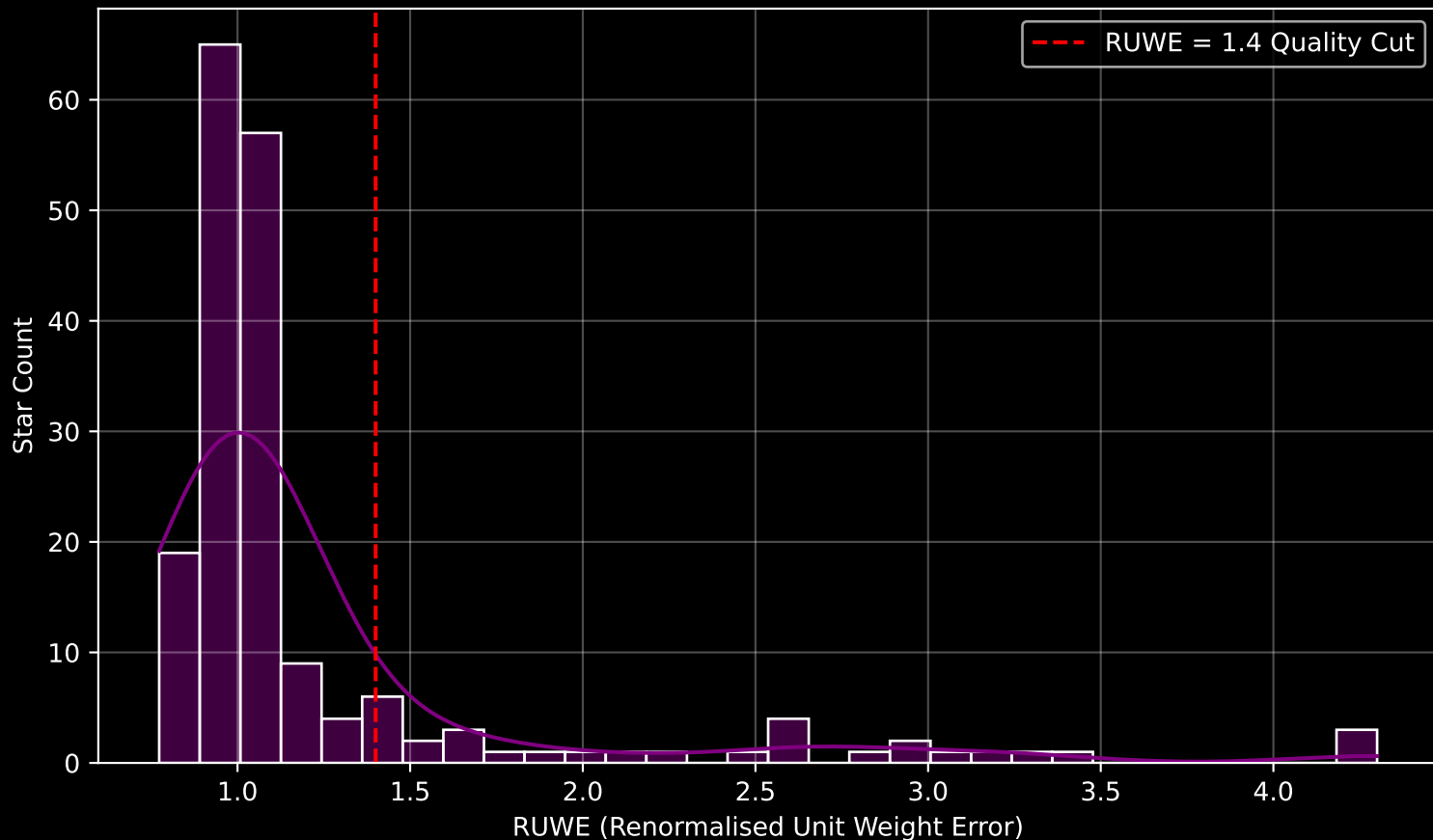
GAPOGEE DR17 Field [066+47_MGA] RUWE Distribution (n= 185)
