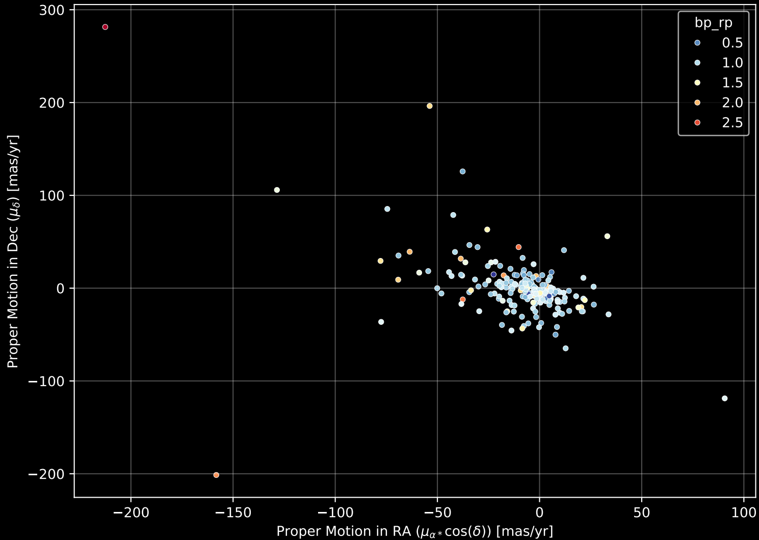
APOGEE DR17 Field: [066+47_MGA] Proper Motion Diagram (n= 198)
