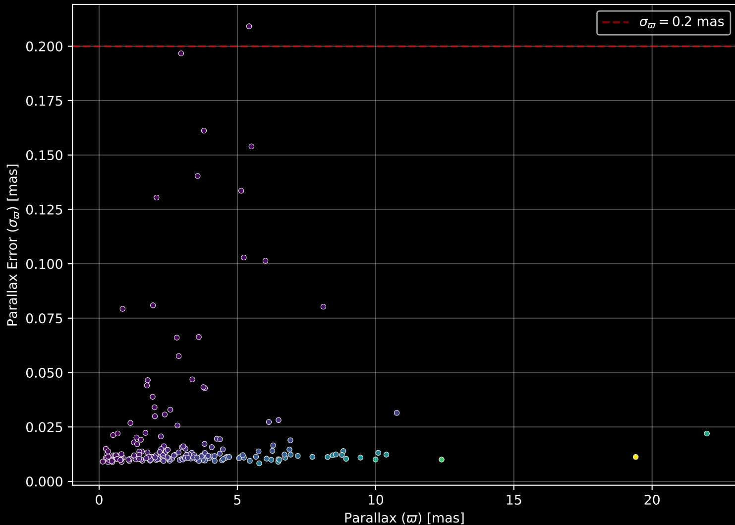
APOGEE DR17 Field: [066+47_MGA] Parallax Quality (n= 198)
