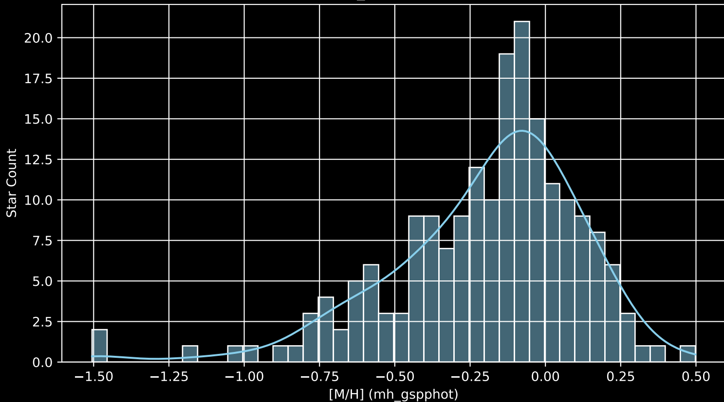
APOGEE DR17 Field: [066+47_MGA [M/H] (mh_gspphot) (n= 194)
