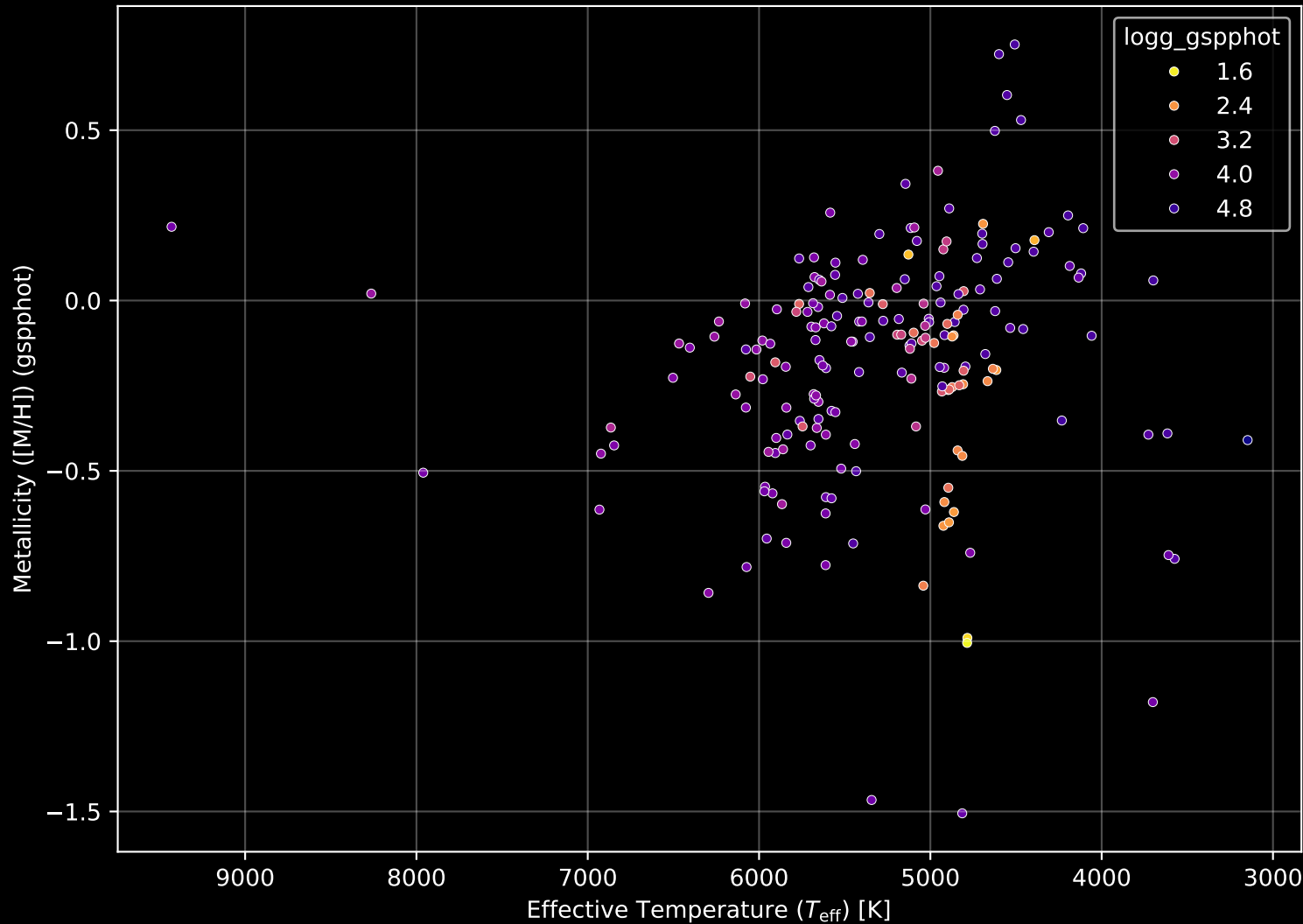
APOGEE DR17 Field: [066+47_MGA] Stellar Population Parameters (n= 198)
